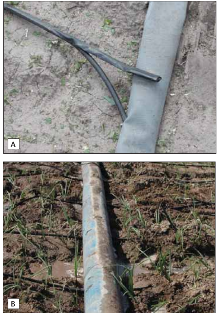
Figure 10. Connecting the drip tape to a manifold above the soil surface with tubing (A) and with a fitting (B).
